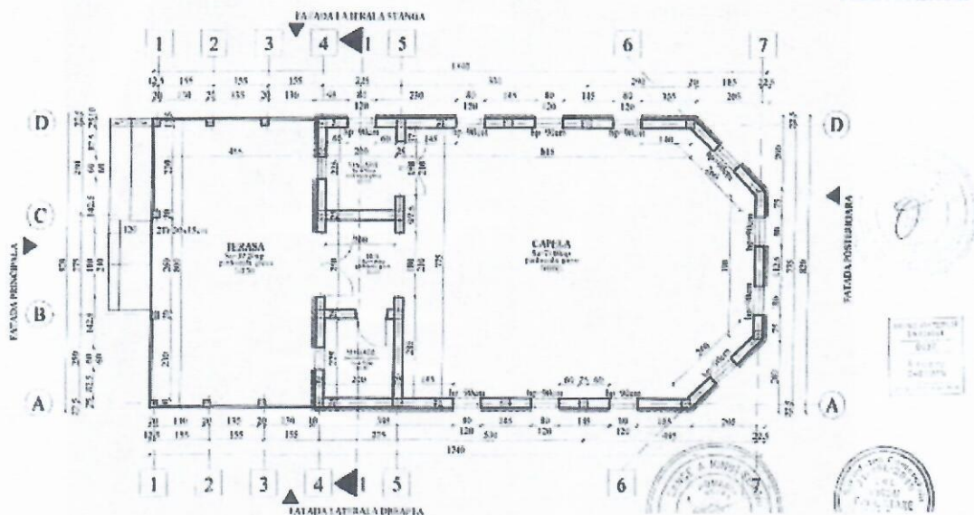
PLAN PARTER
